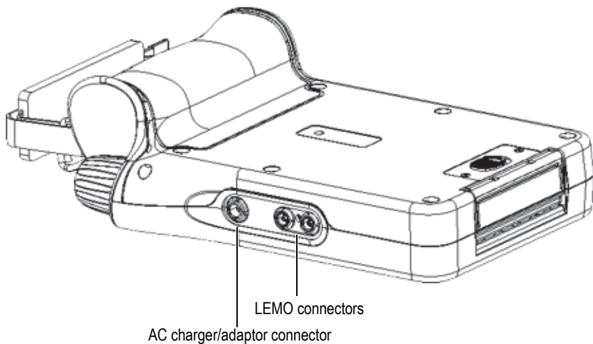
Figure 2-1 External connectors
