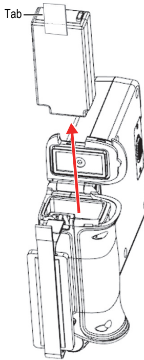
Figure 4-3 Battery removal
